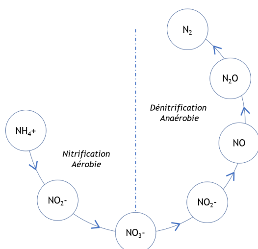
Figure 1 : Processus de nitrification-dénitrification
